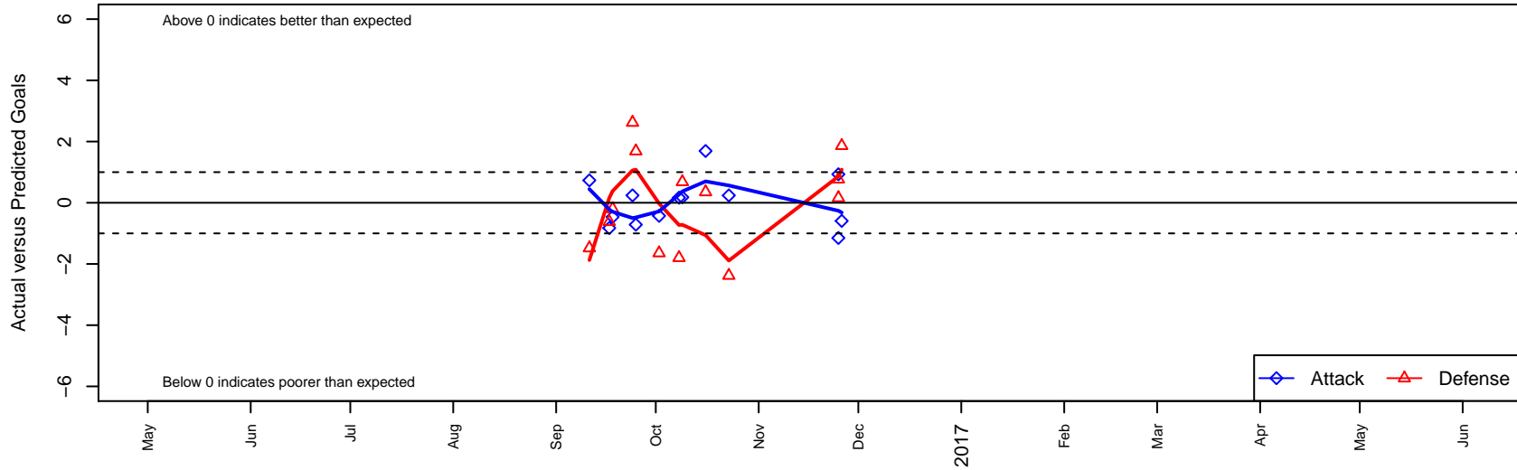
Del Mar Sharks White B02 Dots are actual minus expected GF (blue circles) and GA (red triangles). Blue line is smoothed change in attack strength. Red is smoothed change in defense strength.
